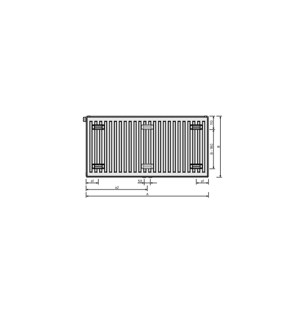
Dimensional Drawing - T6 3010 type 21,22,33, back view
