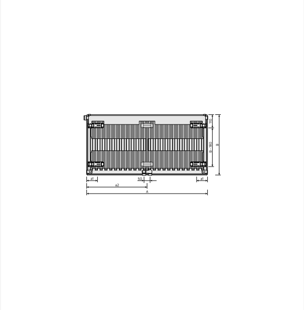
Dimensional Drawing - T6 3010 type 11, back view
