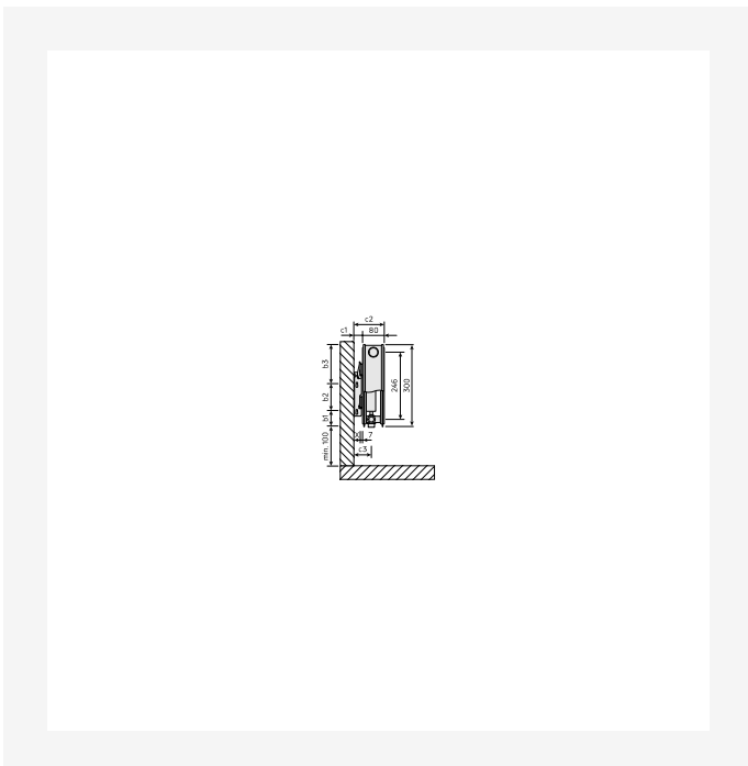
DimensionalDrawing - T6 3010, type 21, profil view
