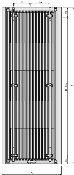
DimensionalDrawing - New_Paros V rear view
