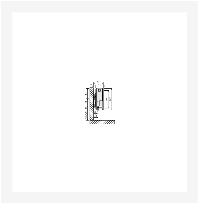
DimensionalDrawing - T6 3010 Plan/Déco type 22 H300, side view
