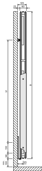
Dimensional Drawing - Vertical, tips 21, skats no sāniem
