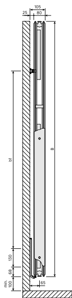
Dimensional Drawing - Vertical, tips 21, skats no sāniem
