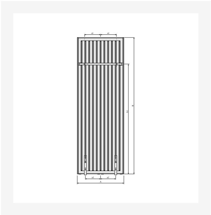
DimensionalDrawing - Vertical ar MCW6 kronšteinim, skats no aizmugures
