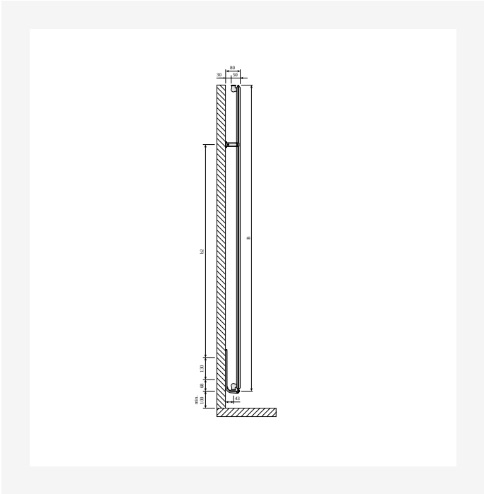
DimensionalDrawing - Vertical, tips 10, skats no sāniem
