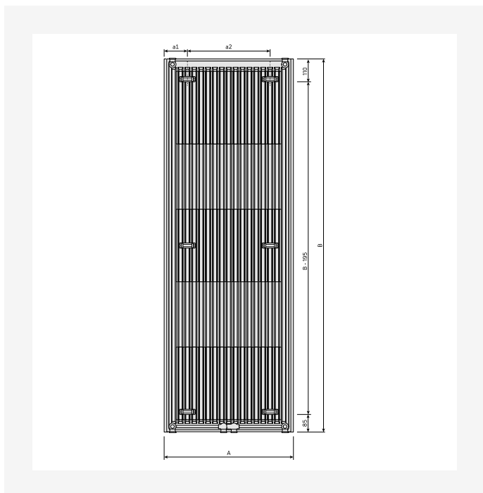
DimensionalDrawing - Tinos V, tips 11, skats no aizmugures
