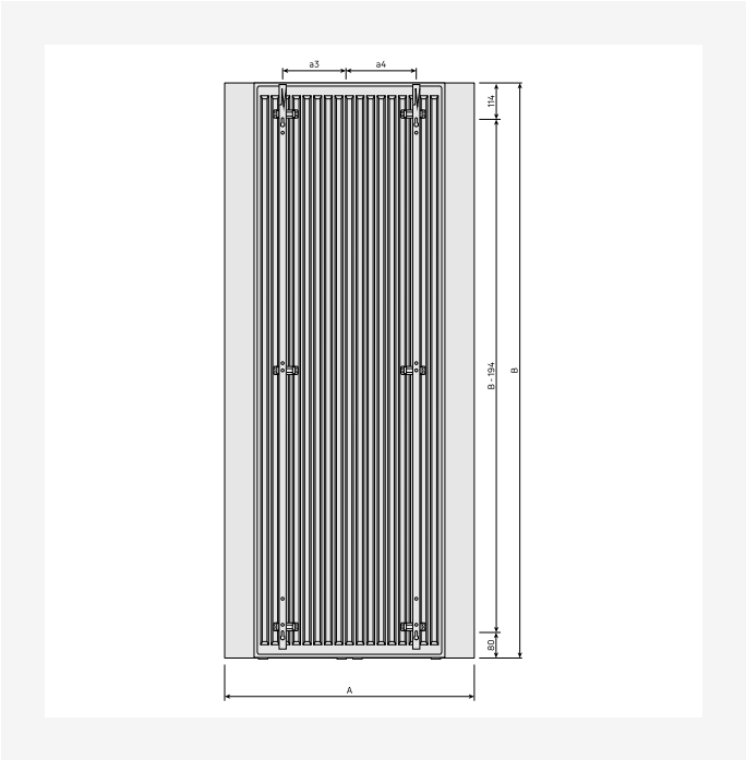
DimensionalDrawing - Paros V, tips 21, skats no aizmugures ar MCWV kronšteinem
