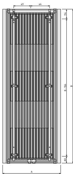
DimensionalDrawing - Paros V, tips 11, skats no aizmugures ar MCWV kronšteinu
