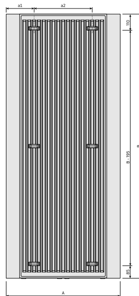
DimensionalDrawing - Paros V, tips 21, skats no aizmugures
