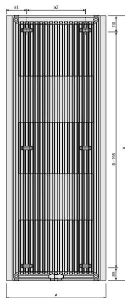
DimensionalDrawing - Paros V, tips 11, skats no aizmugures
