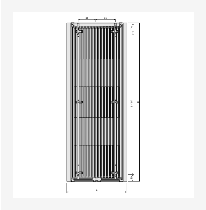
DimensionalDrawing - Paros V, tips 11, skats no aizmugures ar MCWV kronšteinu
