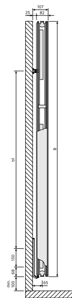
DimensionalDrawing - Kos V / Faro V, tips 21, skats no sāniem
