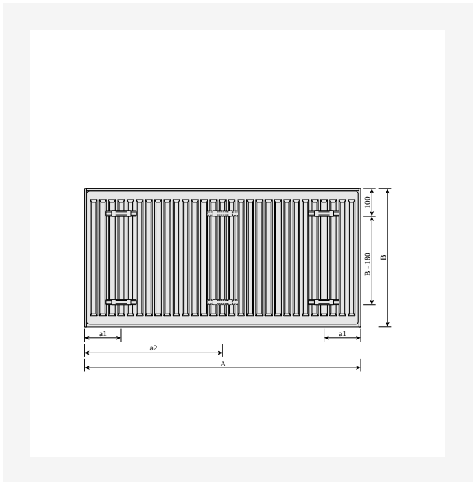
DimensionalDrawing - Plan Compact, skats no aizmugures
