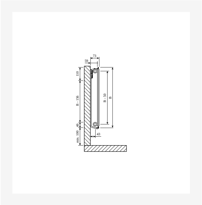
DimensionalDrawing - Hygiene, tips 10, skats no sāniem ar Monclac sienas kronšteinu
