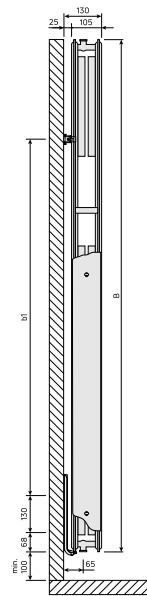
DimensionalDrawing - Vertical, type 22, sidevisning
