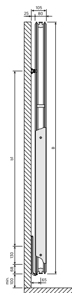
DimensionalDrawing - Vertical, type 20, sidevisning
