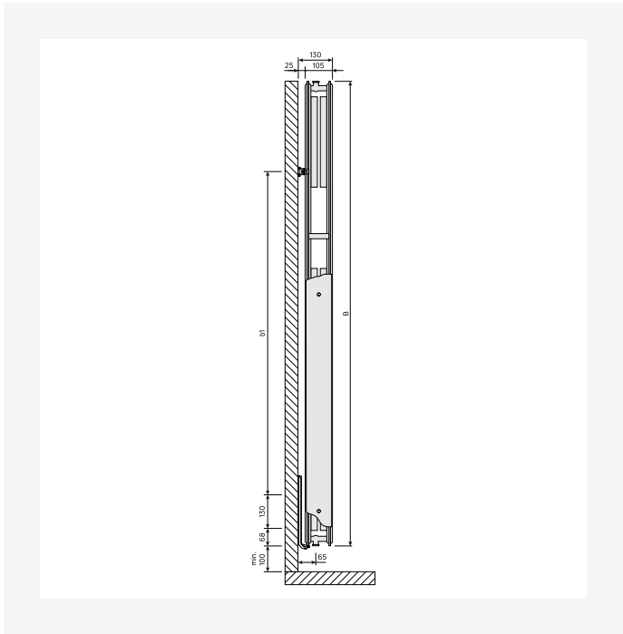
DimensionalDrawing - Vertical, type 22, sidevisning
