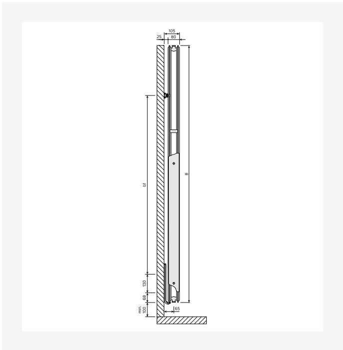
DimensionalDrawing - Vertical, type 20, sidevisning
