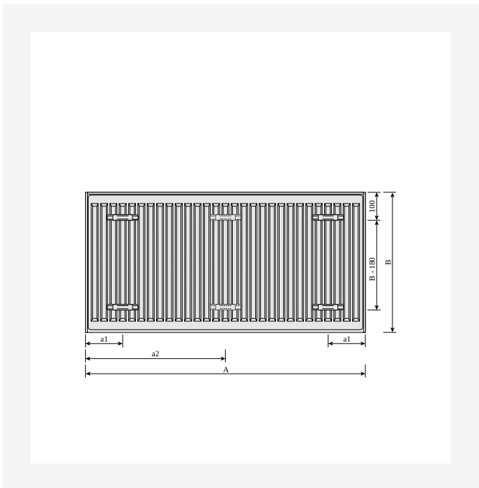
DimensionalDrawing - Plan Compact, bagvisning
