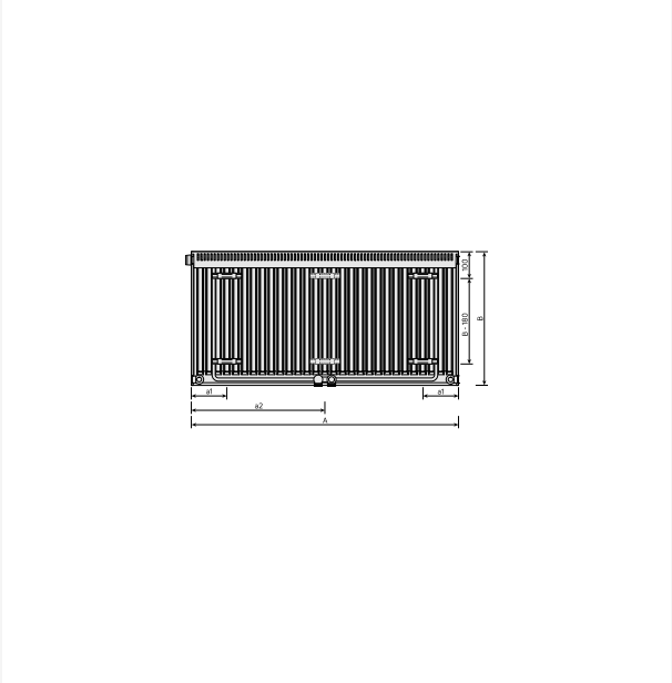
Dimensional Drawing - Flex, type 11, bagfra
