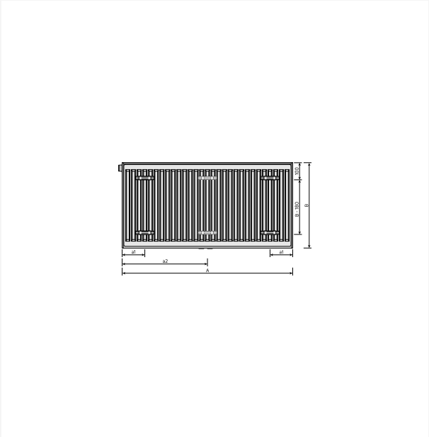
Dimensional Drawing - Flex, typer 21, 22, 33, bagfra
