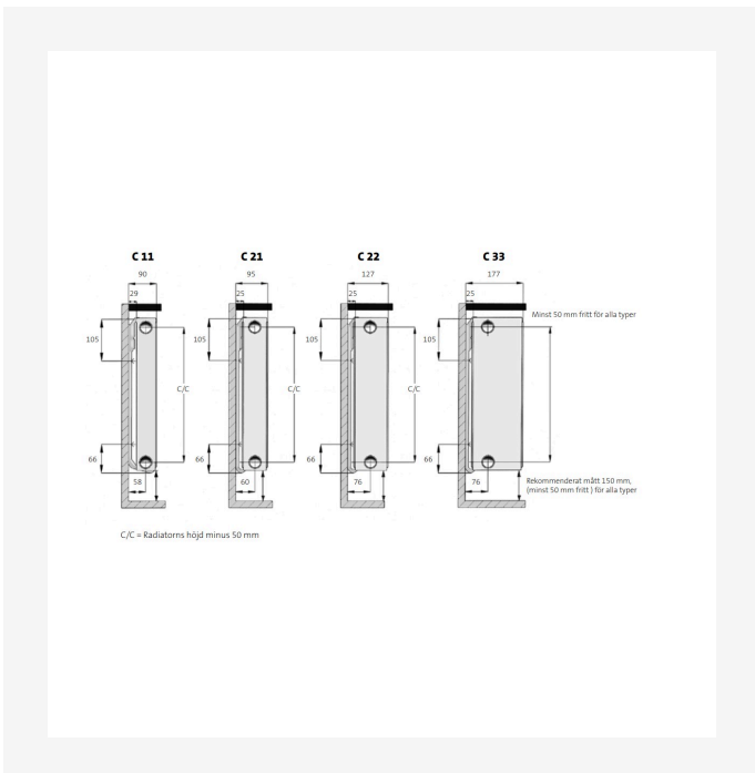
DimensionalDrawing - Installationsmål
