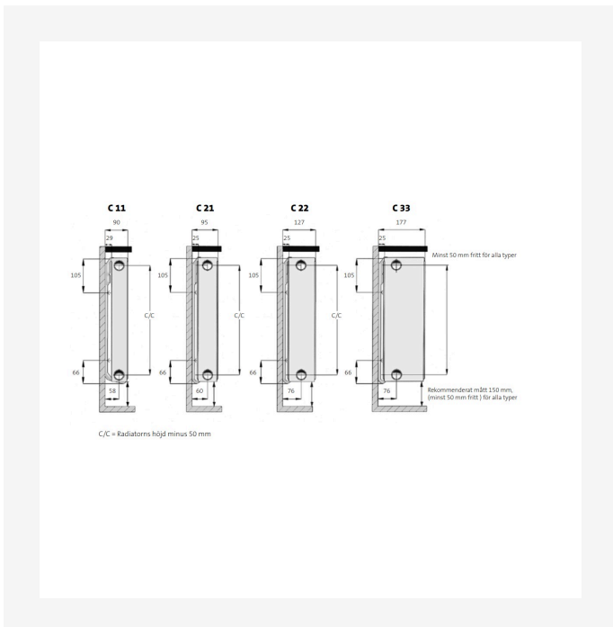
DimensionalDrawing - Installationsmål
