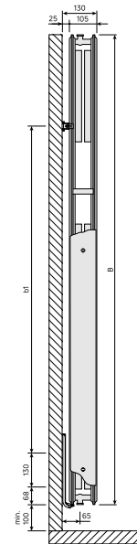
DimensionalDrawing - New_Vertical side view
