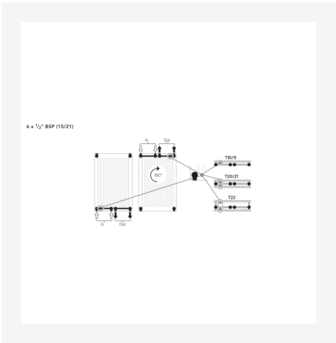
Installation Instructions - Vertical Connection Options
