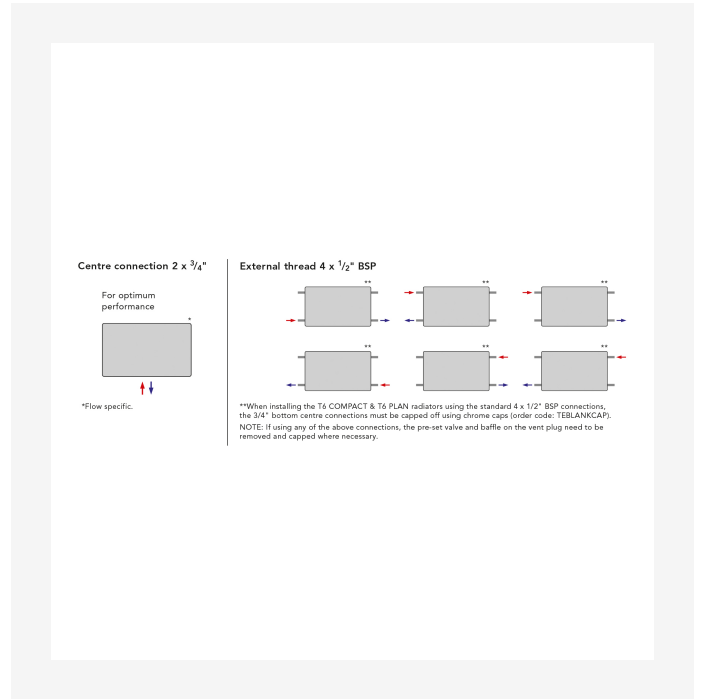
Installation Instructions - Vonova T6 Connection Options
