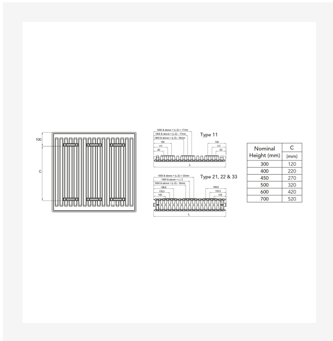
Dimensional Drawing - Select Compact Bracket Positions and Dimensions
