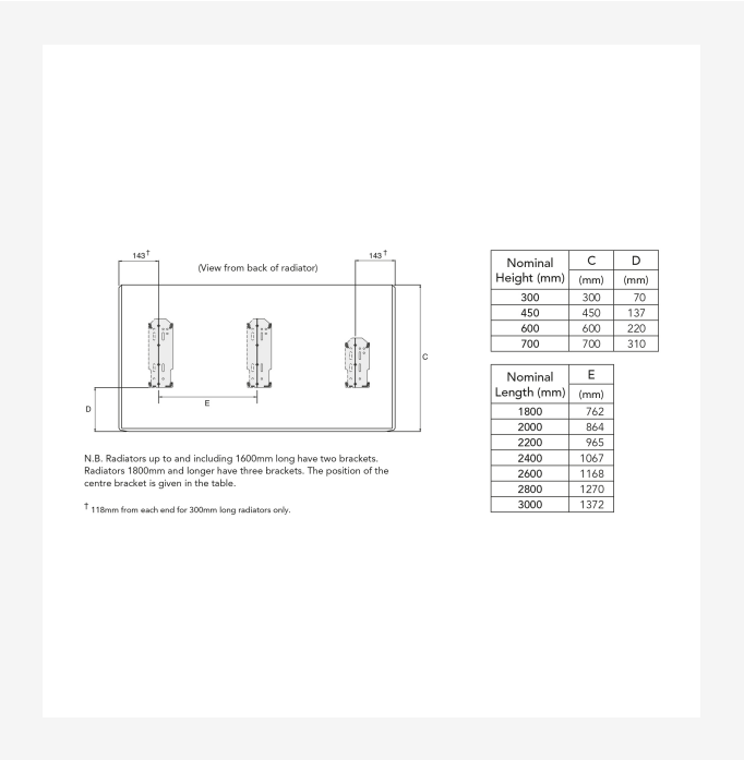
DimensionalDrawing - Premier Metric Bracket Positions and Dimensions
