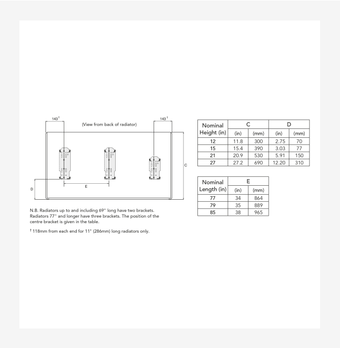
DimensionalDrawing - Premier HE Bracket Positions and Dimensions
