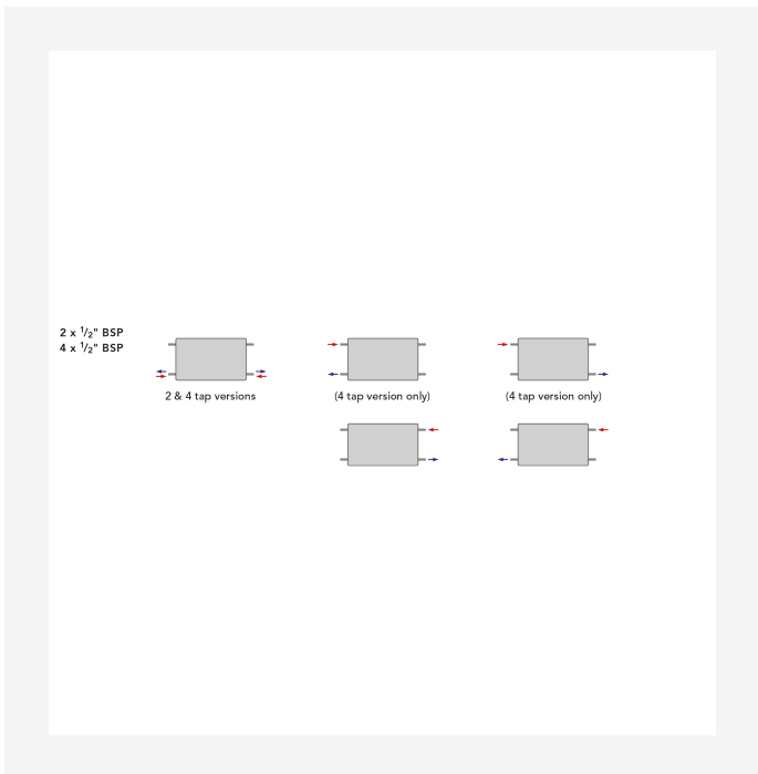
Installation Instructions - Premier HE Connection Options
