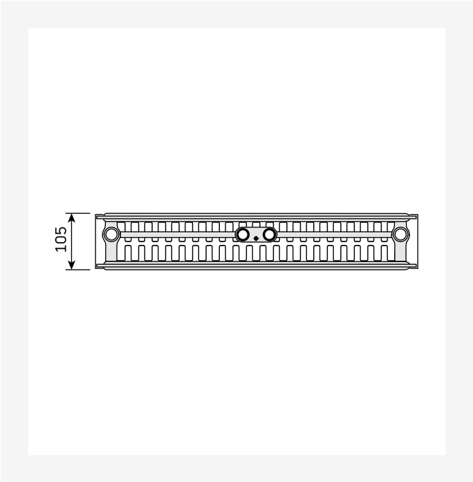
DimensionalDrawing - Vertical typ 22, bottenvy
