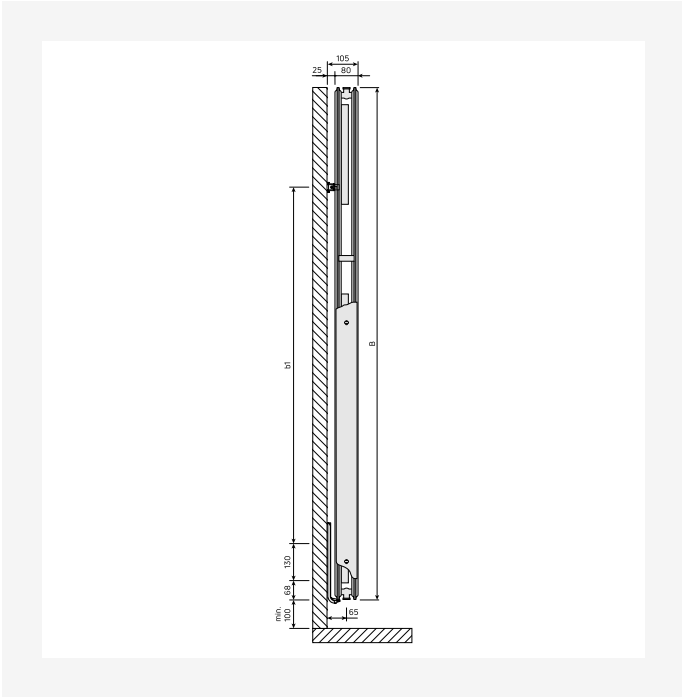
DimensionalDrawing - Vertical typ 21, sidovy
