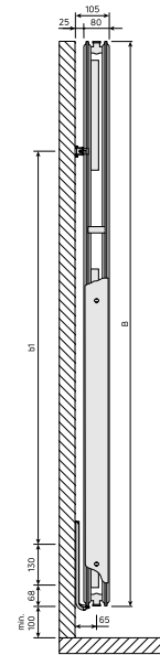
Dimensional Drawing - Vertical typ 21, sidovy
