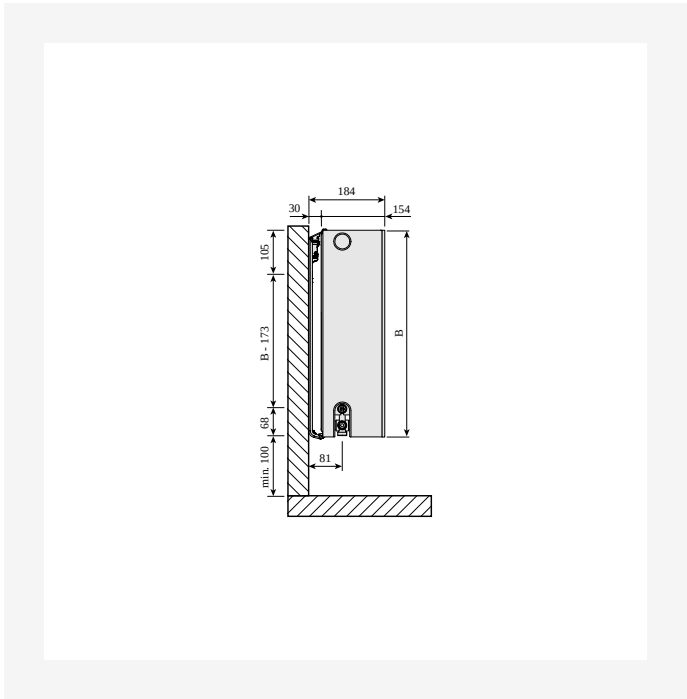
DimensionalDrawing - Thermopanel Plan typ 33, sidovy
