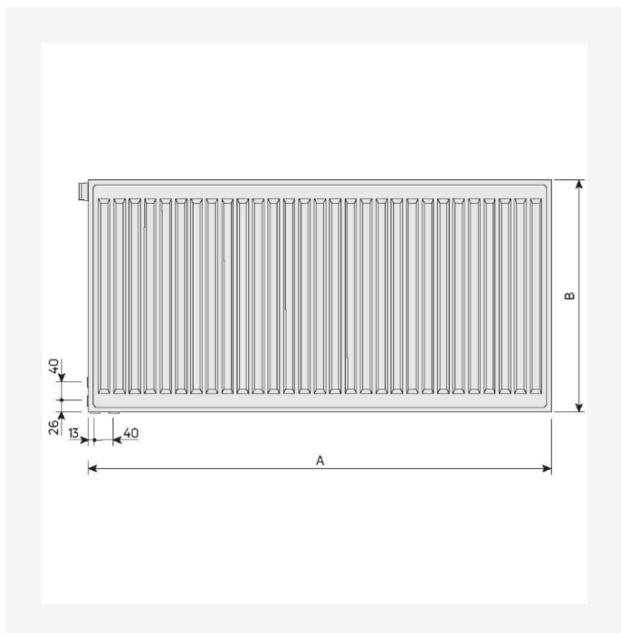
DimensionalDrawing - Thermopanel Hygiene, vänster frontvy
