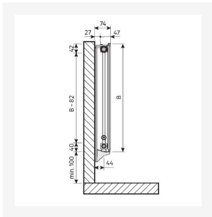
DimensionalDrawing - Thermopanel typ 10, sidovy
