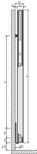
DimensionalDrawing - New_Kos V-Faro V side view
