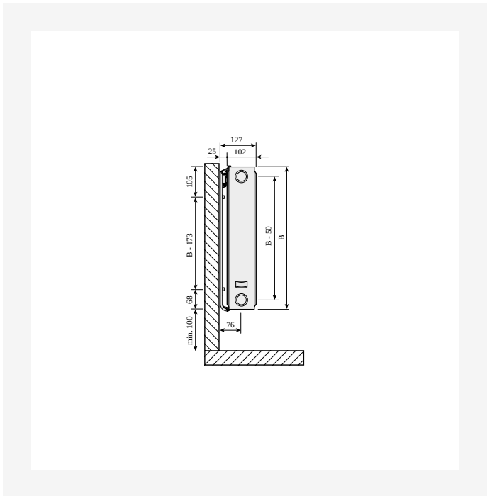
DimensionalDrawing - Compact, typ 22 sidovy
