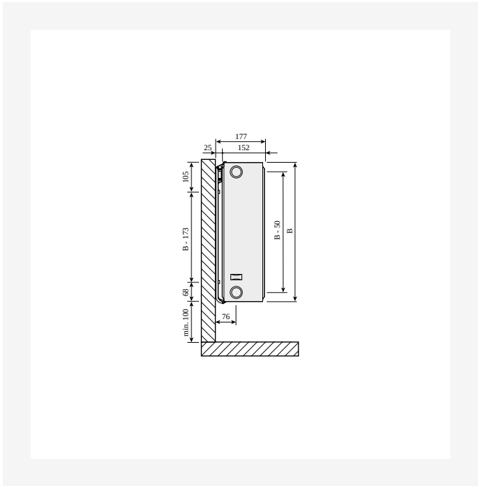
DimensionalDrawing - Compact, typ 33 sidovy
