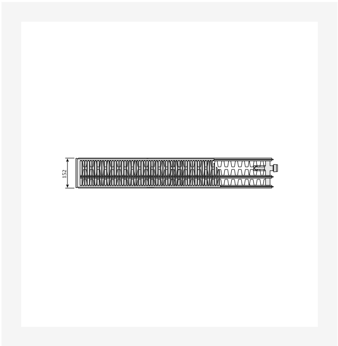
DimensionalDrawing - Tip 33
