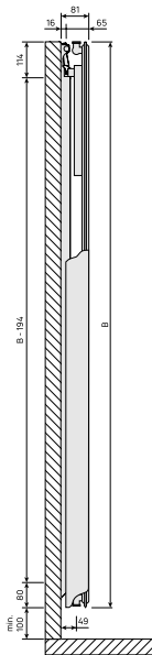
DimensionalDrawing - New_Tinos V-Paros V side view
