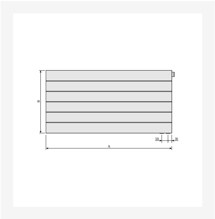
DimensionalDrawing - Ramo Ventil Compact, front view right
