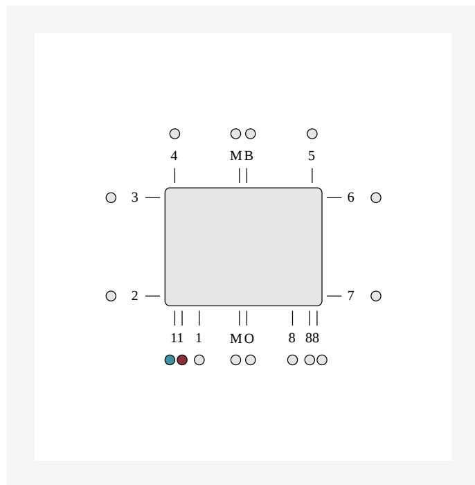
Schiță dimensională - Hor-connection-ETIM-11-in-right-out-left-1219
