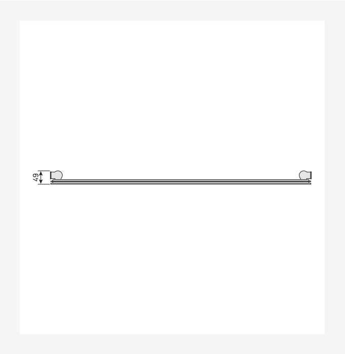
DimensionalDrawing - Plan Hygiene, tip 10, vedere de sus
