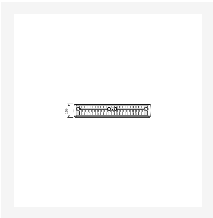
DimensionalDrawing - Kos V and Faro V, type 22, vedere de sus
