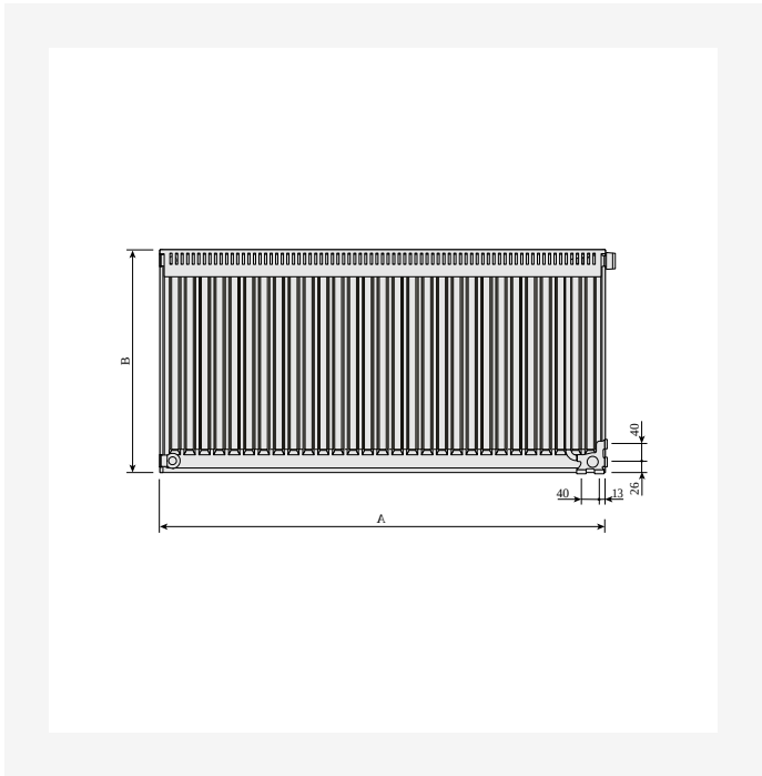
DimensionalDrawing - Termopanel type 11, venstre bakfra
