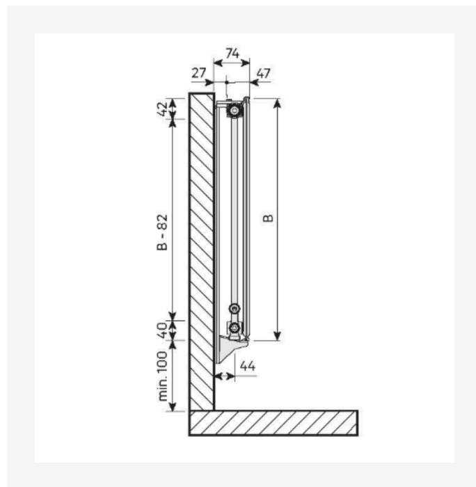
DimensionalDrawing - TPV4 Hygiene (SE)_v4_SV_T10 (1)
