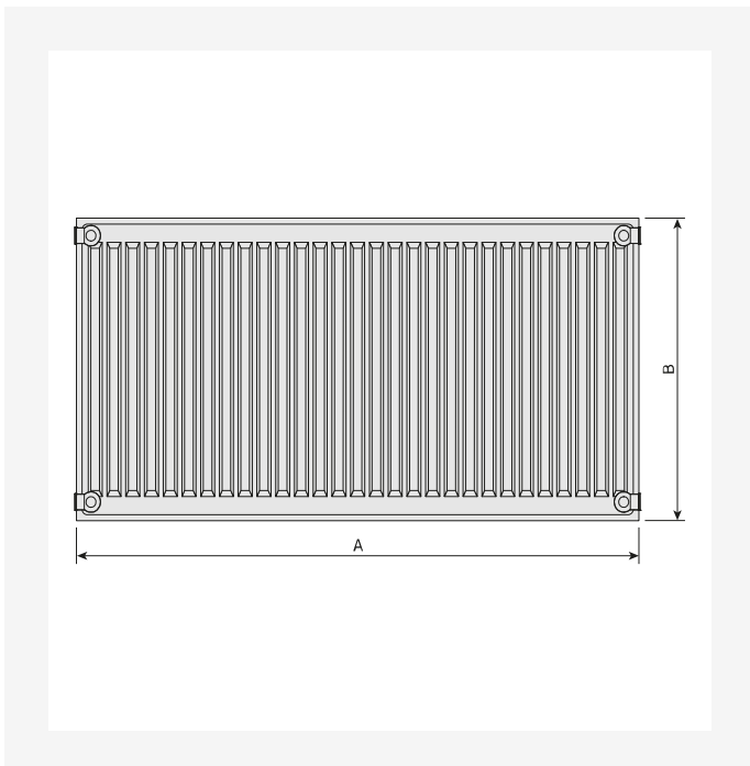
DimensionalDrawing - PR-Hygiene-RV-T10-0924
