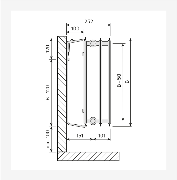
Dimensional Drawing - Hygiene, type 30 sidevisning
