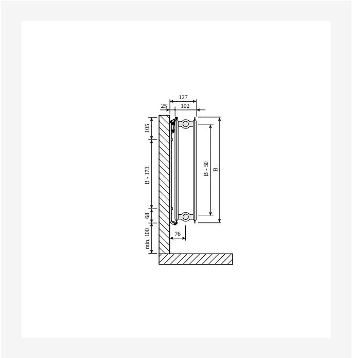
Dimensional Drawing - Hygiene, type 20 sidevisning
