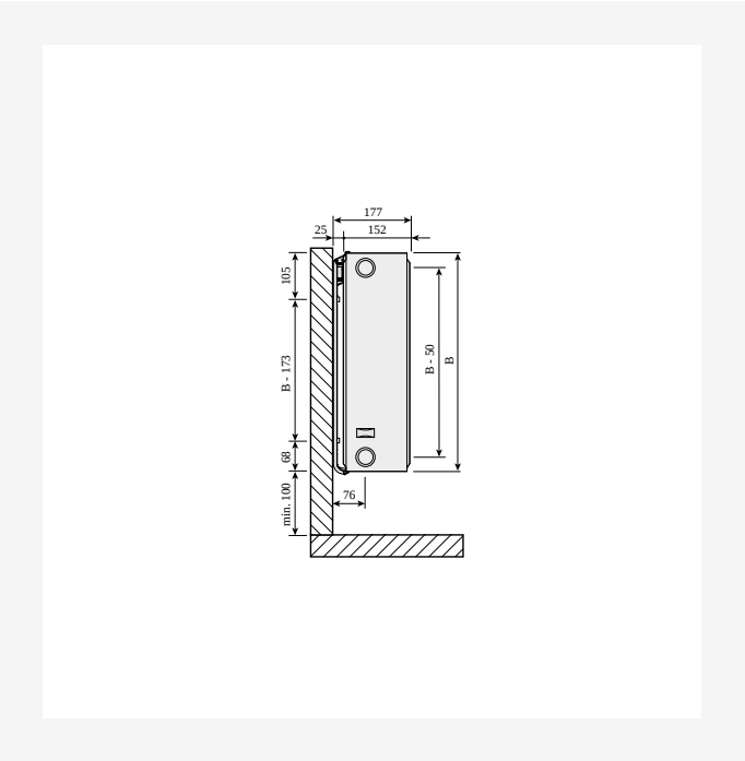
Dimensional Drawing - Compact, type 33 sidevisning
