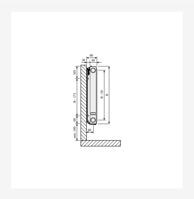
Dimensional Drawing - Compact, type 11, sidevisning
