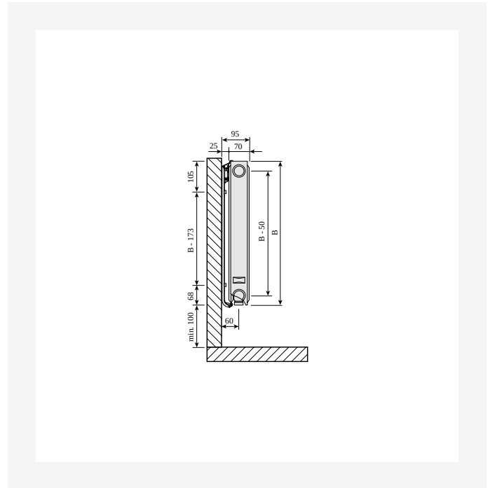
Dimensional Drawing - Ventil Compact, type 21s, skats no sāniem ar Monclac sienas kronšteiniem
