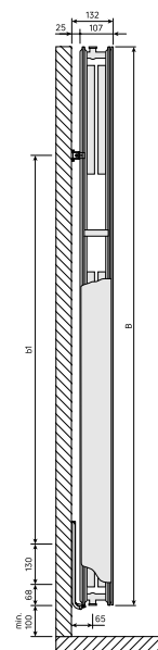
DimensionalDrawing - Kos V / Faro V, tips 22, skats no sāniem
