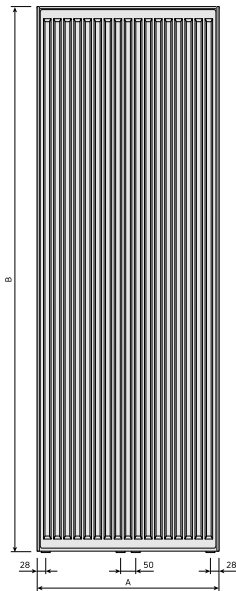
DimensionalDrawing - Vertical ab 2024 Frontansicht Typen 20, 21, 22
