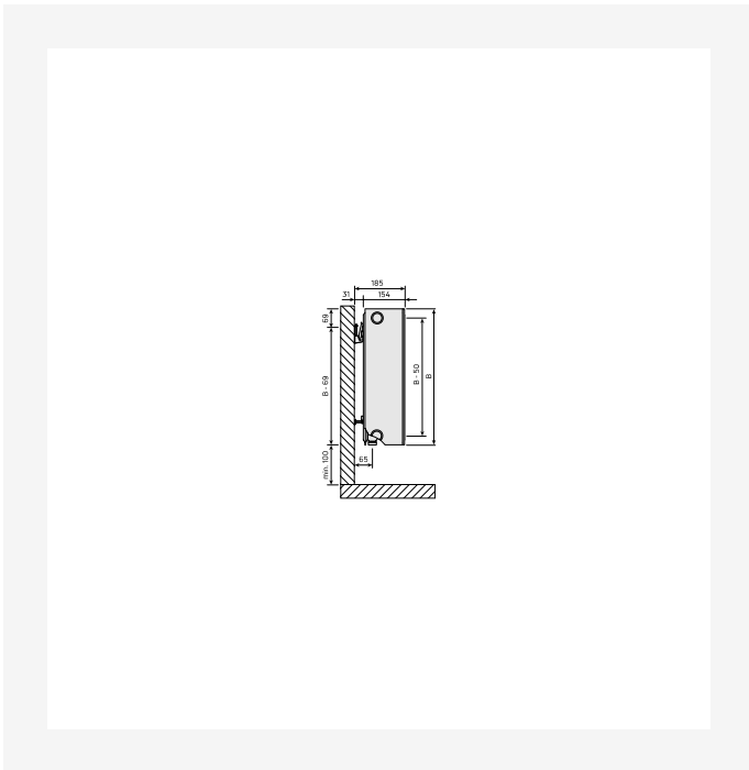
DimensionalDrawing - Plan Ramo Flex sideview typ 33
