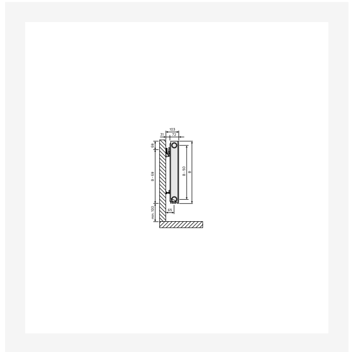
DimensionalDrawing - Plan, Ramo Flex, Sideview, type 21
